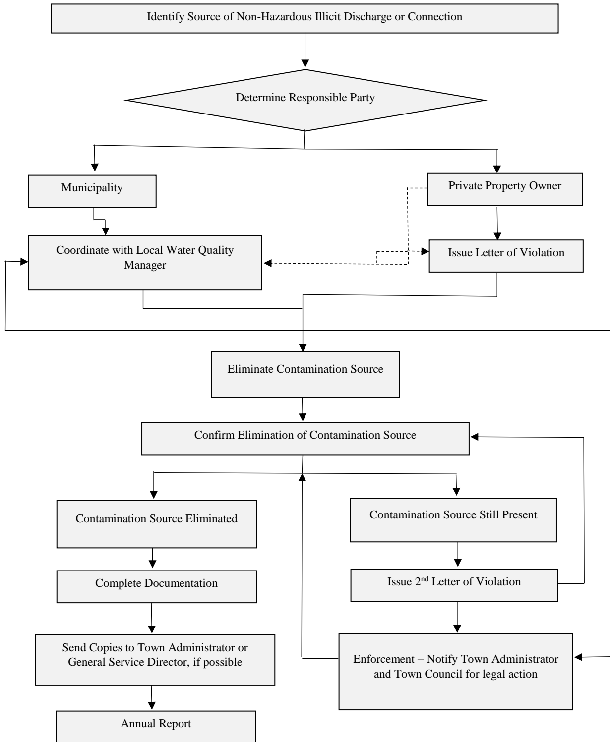
FIGURE 2 Escalating Process for Removing or Correcting an Illicit Discharge
